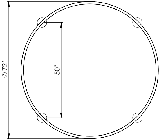
RIGID STEM OPTION (T30)
